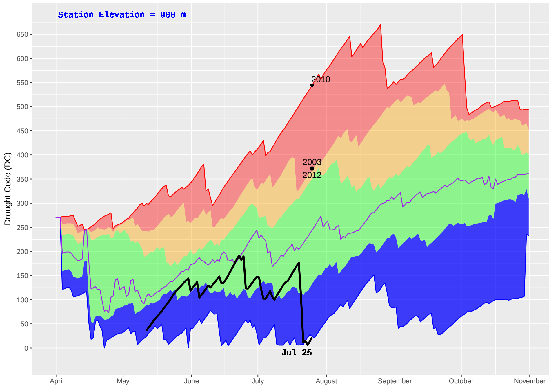
NOEL (437) : Historical (1993–2016) and Current (2018) Noon Drought Code (DC)
